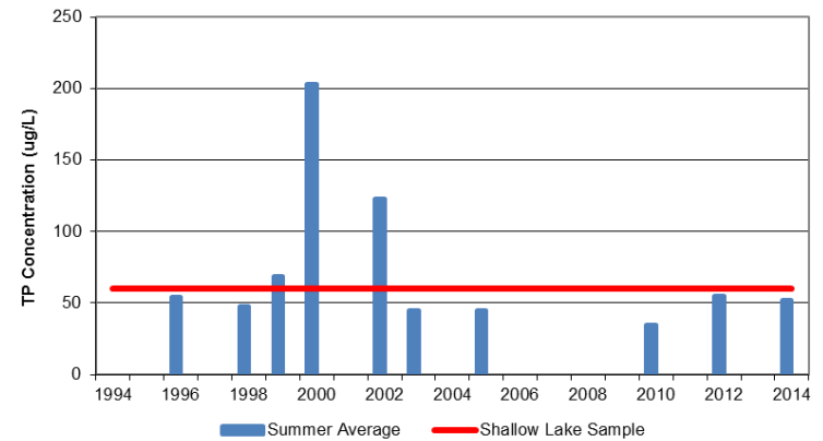
LowerTwin Lake Total Phosphorus
