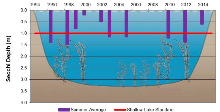
Lower Twin Lake Transparency
